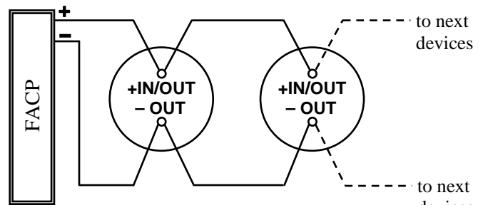
ND-751T-E Wiring Diagram
