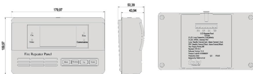
Fig.1 LCD Repeater Panel Structure
