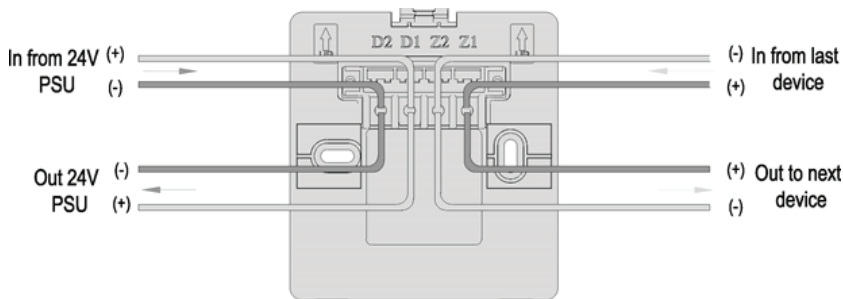
Fig.2 Wiring Details
